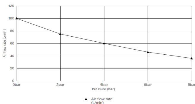
HC550D air flow rate curve
