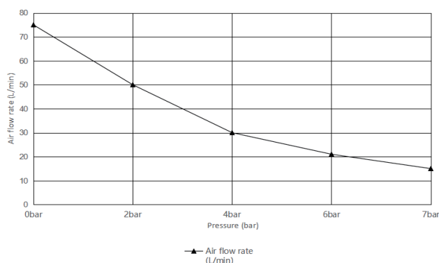
HC280D air flow rate curve
