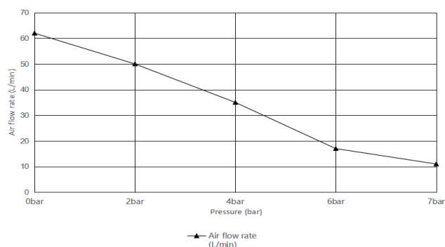
HC210D air flow rate curve
