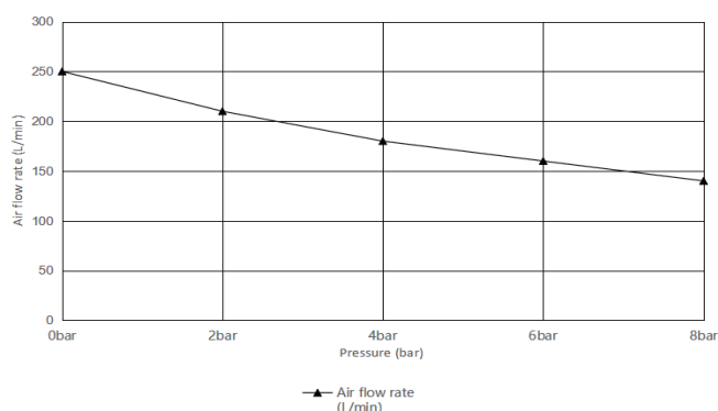
HC1500D air flow rate curve
