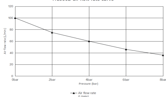
HC550D air flow rate curve
