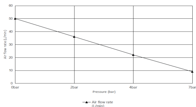
HC100D air flow rate curve
