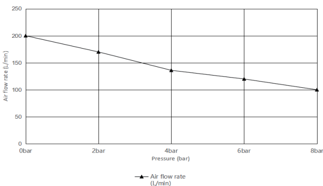
HC1100D air flow rate curve
