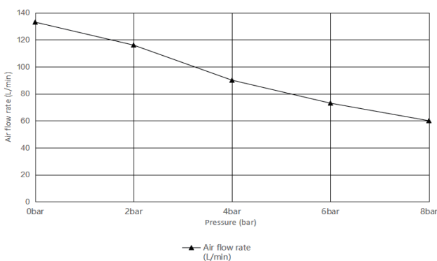
HC750D air flow rate curve
